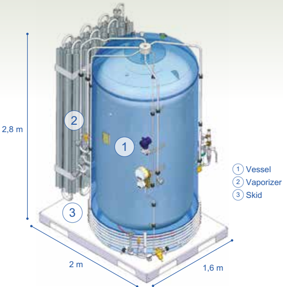
Skid Tank 3000 L 16 barg (PED compliant)
